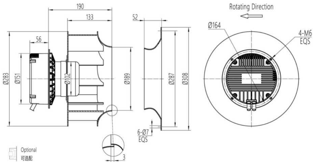
EC Backward Curved Centrifugal Fans 280mm
